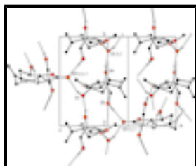
Fig. 2. A view of the hydrogen-bonding network. Hydrogen atoms not involved in the O—H...O interactions have been omitted.
