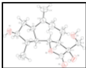
Fig. 1. Molecular structure of cynaratriol represented showing displacement ellipsoids at the 50% probability level.
